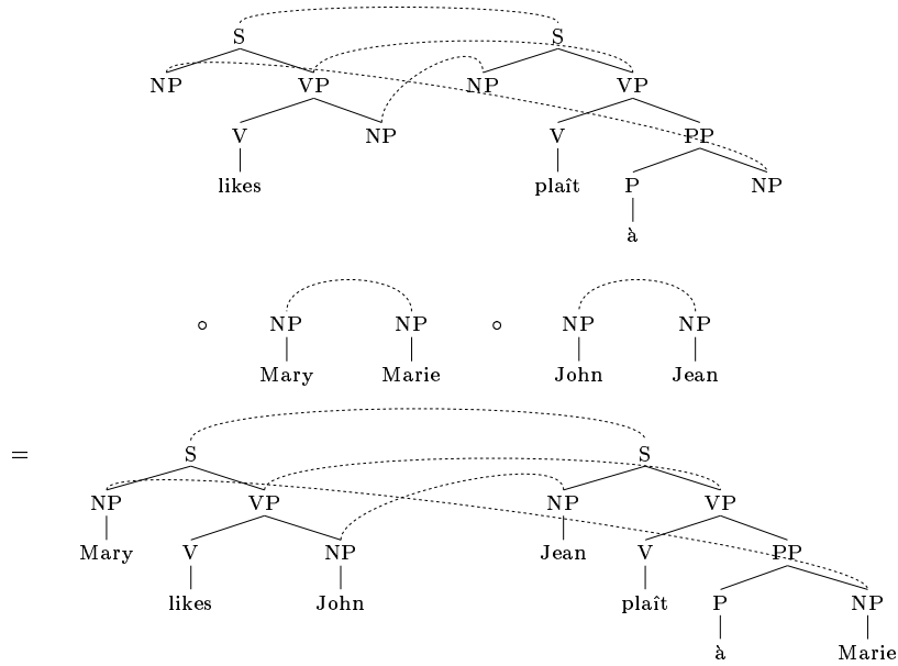
FIGURE 1 Correct derivation of Mary likes John \leftrightarrow Jean plaît à Marie in DOT2
