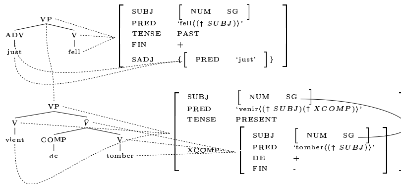
FIGURE 3 The just \longleftrightarrow venir de headswitching case in LFG-DOT3
