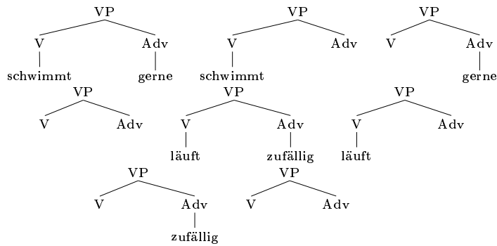
FIGURE 2 The monolingual DOP VP-fragments for a treebank built from the German examples in (3)
