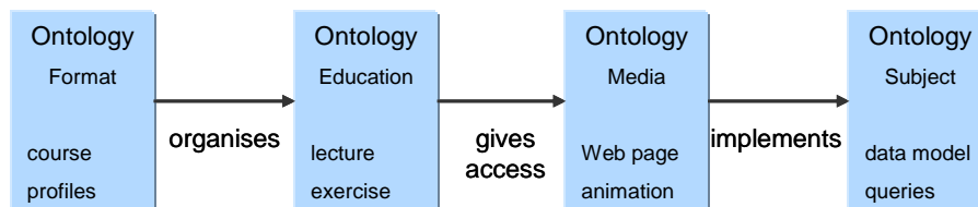
Fig. 2. Ontology Hierarchy.
