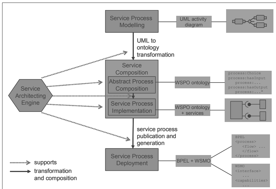
Figure 1 Overview of the ontology-based service architecture technique
