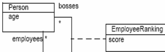
Figure 7.2 - Navigating recursive association classes
