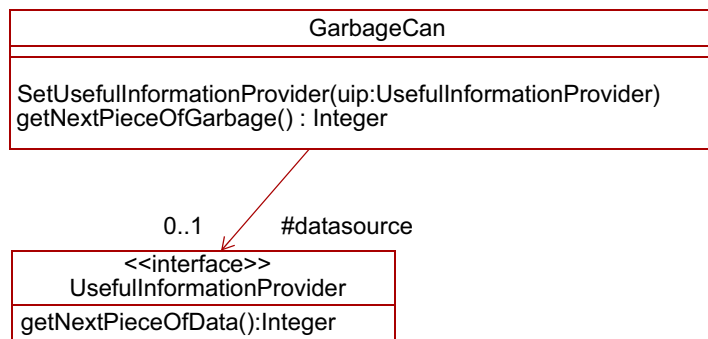
Figure 7.5 - OclMessageExample
