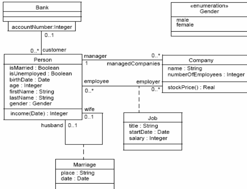
Figure 7.1 - Class Diagram Example
