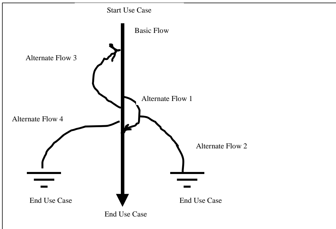
Figure 1: Basic Flow of Events and Alternate Flows of Events for a Use Case
