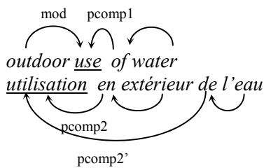
Figure 2. Ambiguous propagation from head nouns
