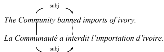
Figure 1. Syntax-based propagation
